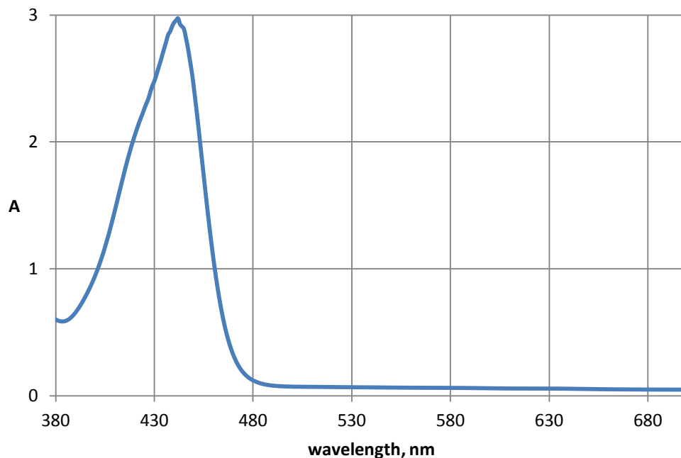
Absorbance spectrum Epolight 5854 in polycarbonate
